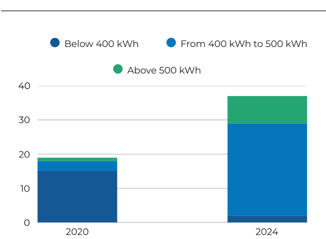
Bus Distribution 12 meters vs. battery capacity 2
