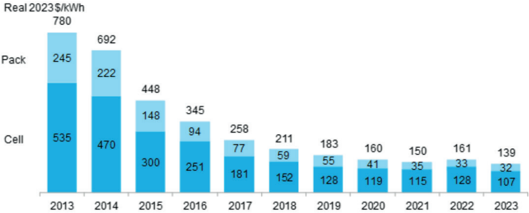
Volume-weighted average prices of lithium-ion battery packs and cells
